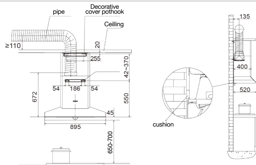
Product installation diagram
