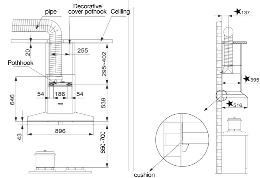
Product installation diagram (★ is the distance from the wall)
